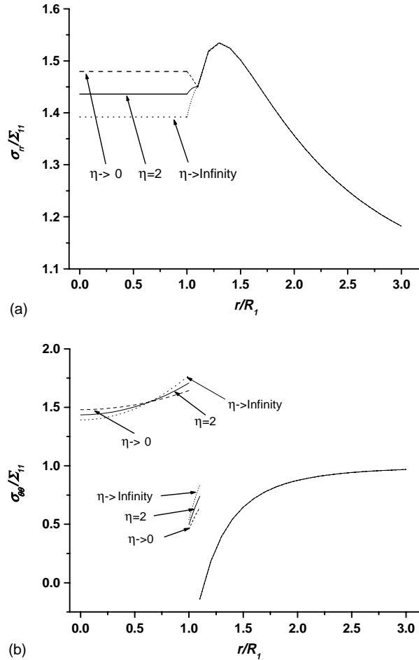
Fig. 3. Variation of stresses for different values of parameter \eta = R_1/c_2 : (a) \sigma_{rr}/\Sigma_{11} along \theta = 0 ; (b) \sigma_{\theta\theta}/\Sigma_{11} along \theta = \pi/2 .
