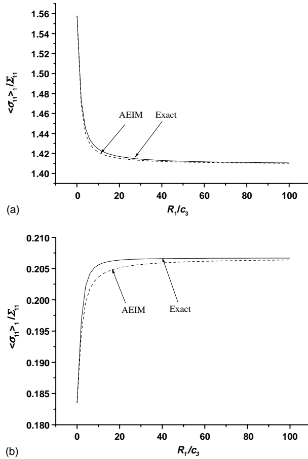
Fig. 6. Comparison of the average stress in a fiber evaluated by exact method and by AEIM method for (a) a hard fiber \mu_1:\mu_3 = 6.4 ; (b) a soft fiber \mu_1:\mu_2 = 0.064 .
