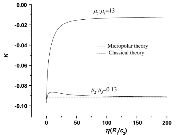
Fig. 4. Influence of fiber's diameter on stress concentration factor for different values of \mu_2:\mu_3 .
