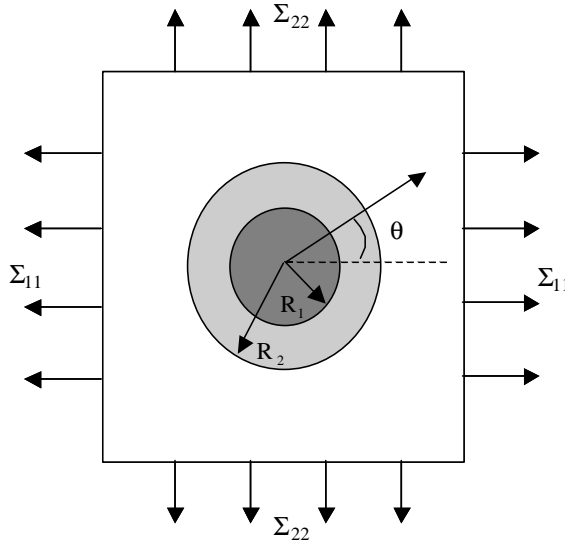
Fig. 2. Sketch of a three-phase model.
