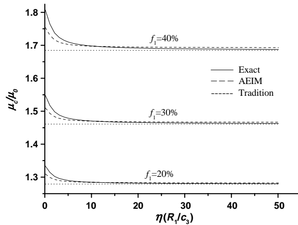
Fig. 7. Effective in plane shear modulus as a function of parameter \eta = R_1/c_3 for different volume fractions of fiber.
