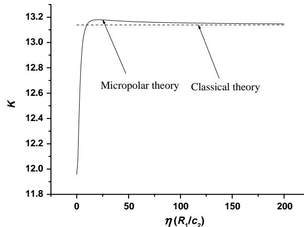
Fig. 5. Influence of void's size on the stress concentration factor for \mu_2:\mu_3 = 13.0 .
